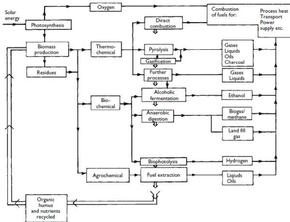
Figure 2.9 Biofuel production process
