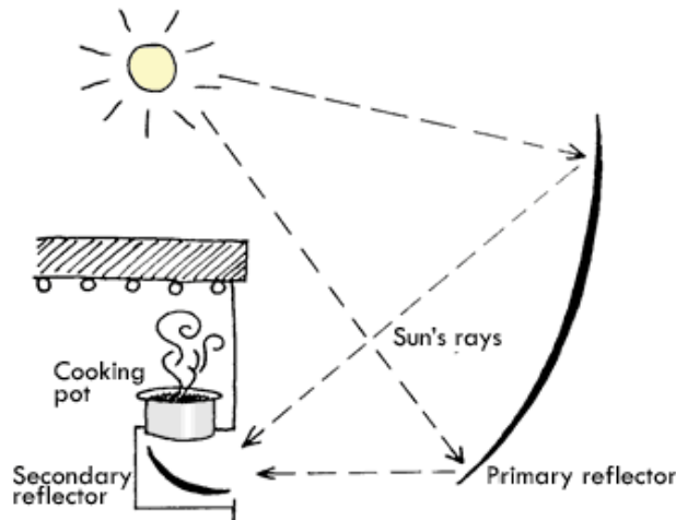
Figure 2.3 concentrating type solar cooker
